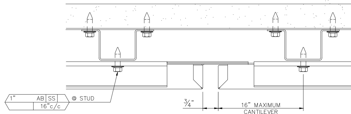
VERTICAL JOINT
