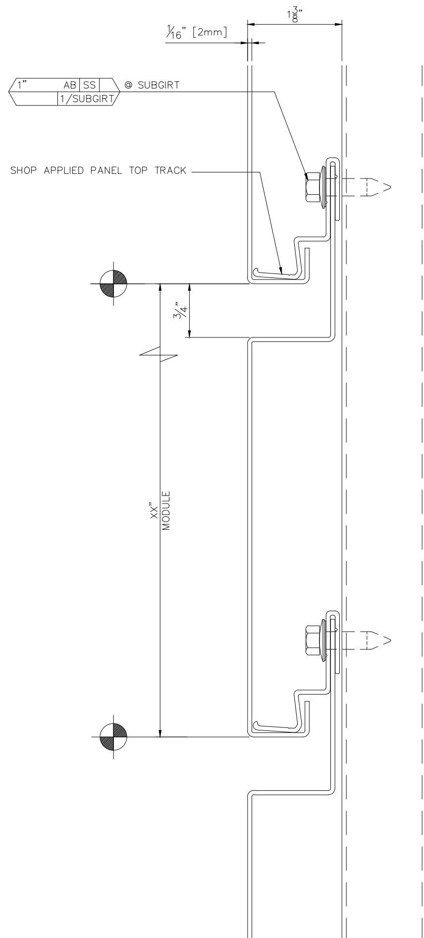
HORIZONTAL PANEL
